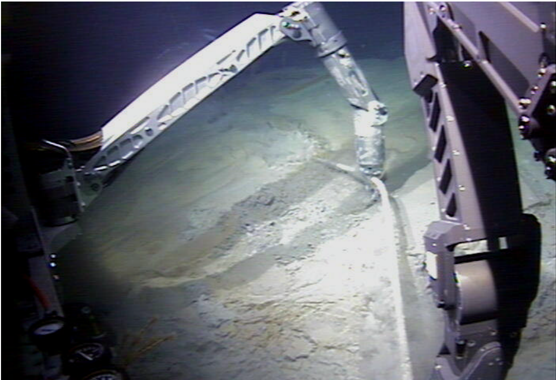
Figure 4: HUGO cable grab with Jason II
