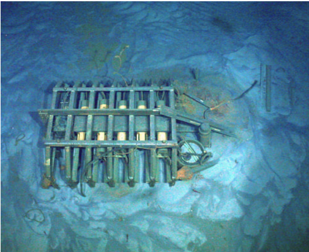
Figure 2: HUGO Approach
