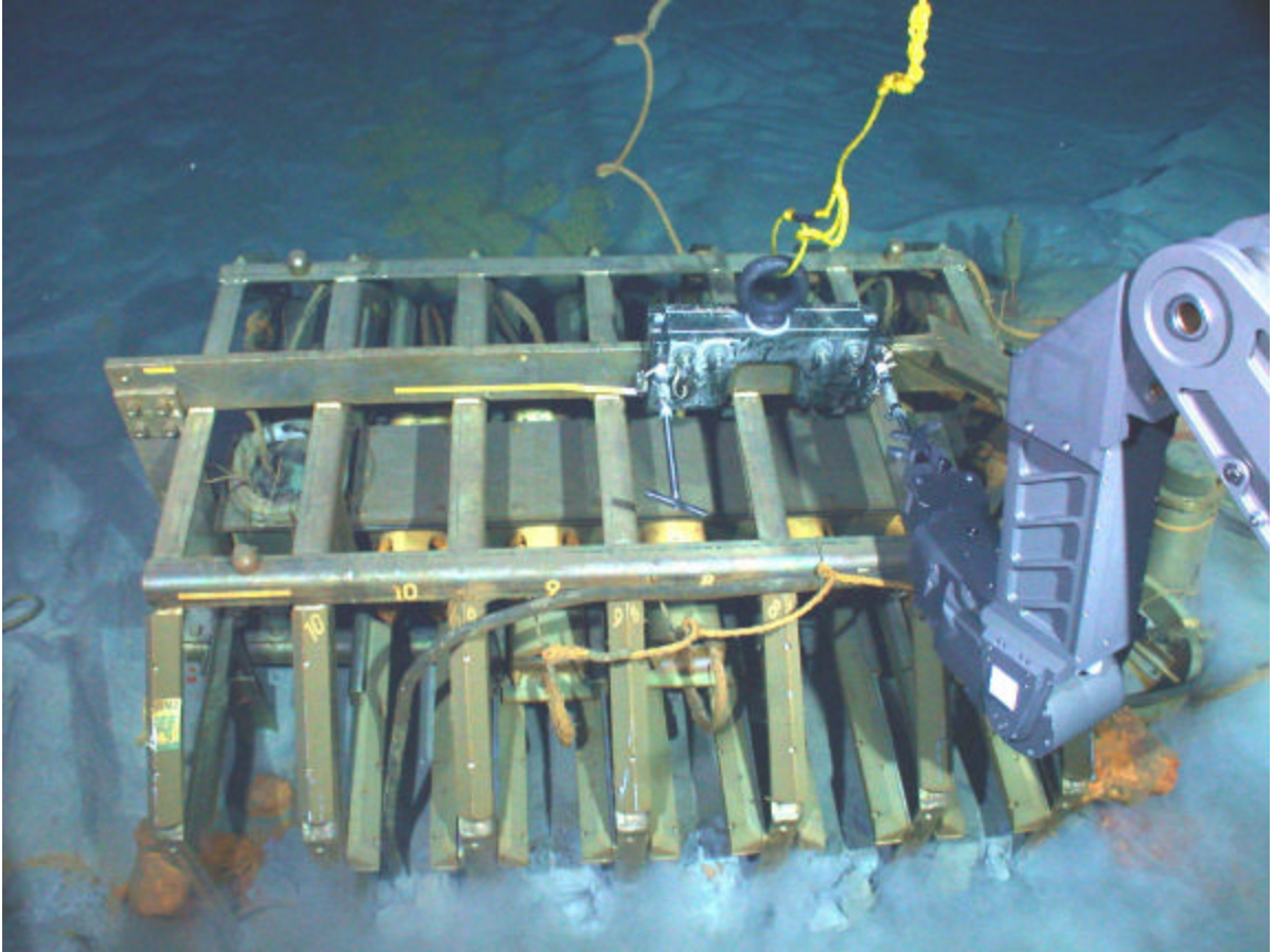
Figure 3: Jason II hook & lock to HUGO
