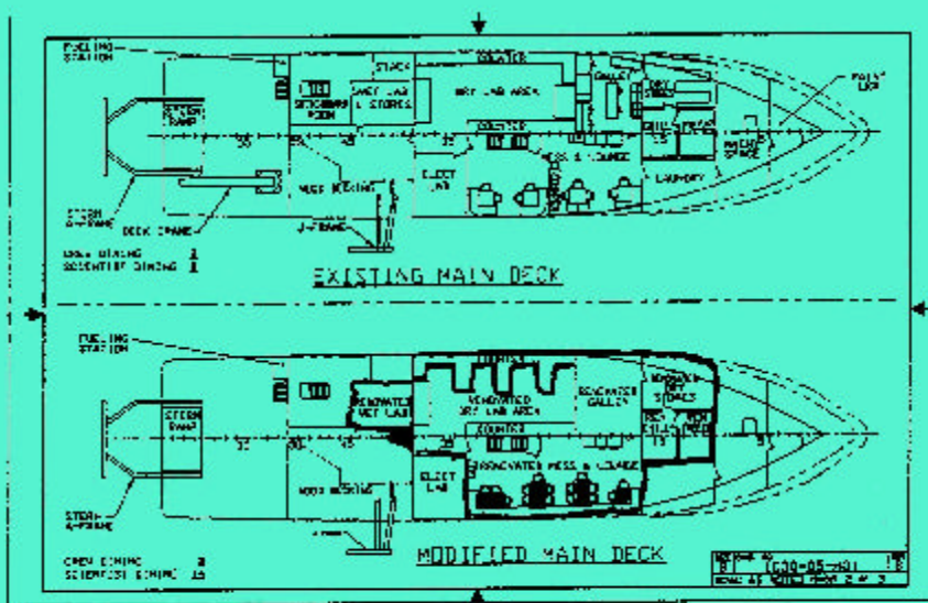
Figure 2. Existing configuration of the main deck and proposed modifications.
