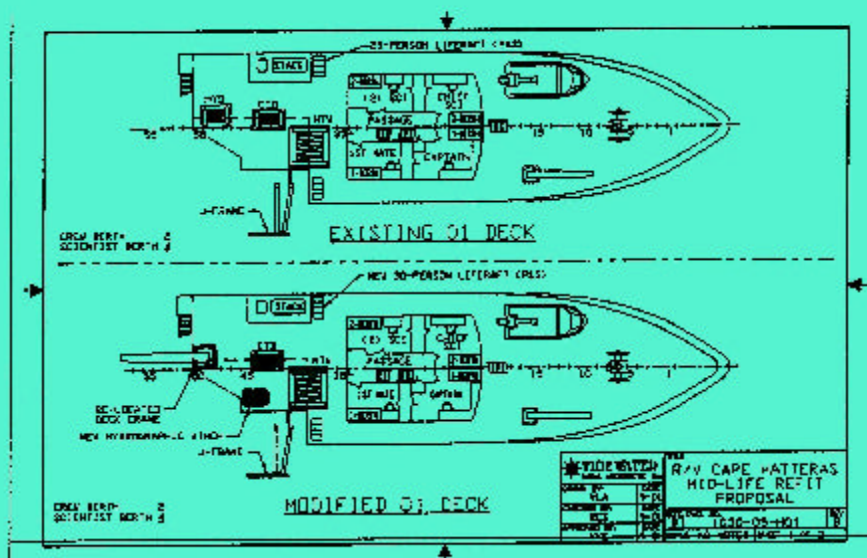
Figure 1. Existing configuration of the 01 deck and proposed modifications.
