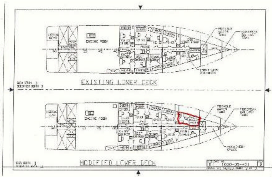
Figure 3. Existing configuration of the lower deck and proposed modifications.
