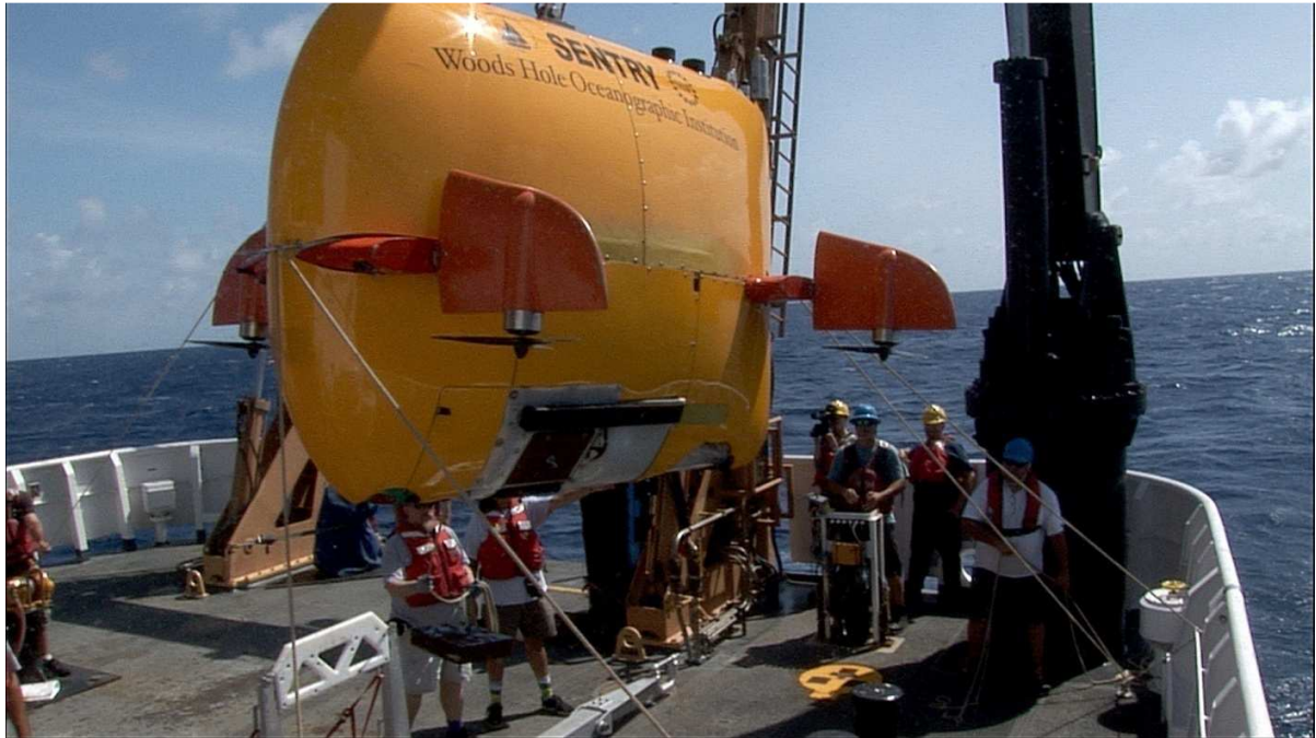
Figure 42 - Sentry is lifted up from the cradle and out towards the rail.
