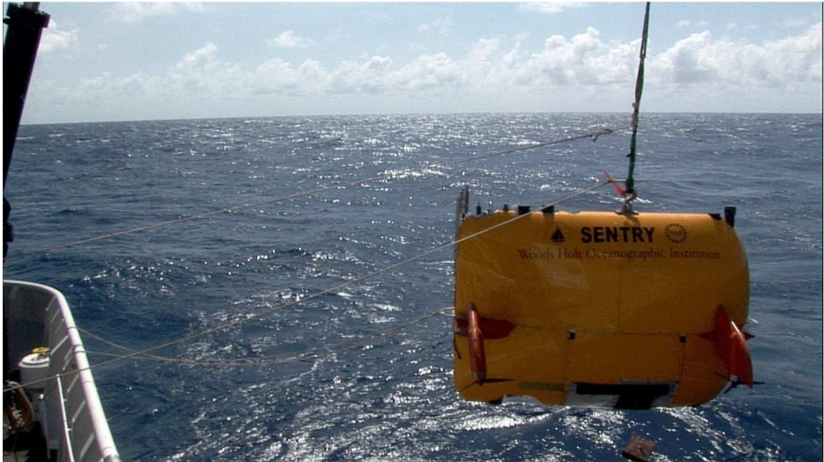
Figure 44 - Sentry continues to move outboard, the aft tagline is used to point the vehicle away from the vessel, then is slipped right before the vehicle enters the water. As soon as the pin is unloaded, it is pulled and the vehicle descends freely.
