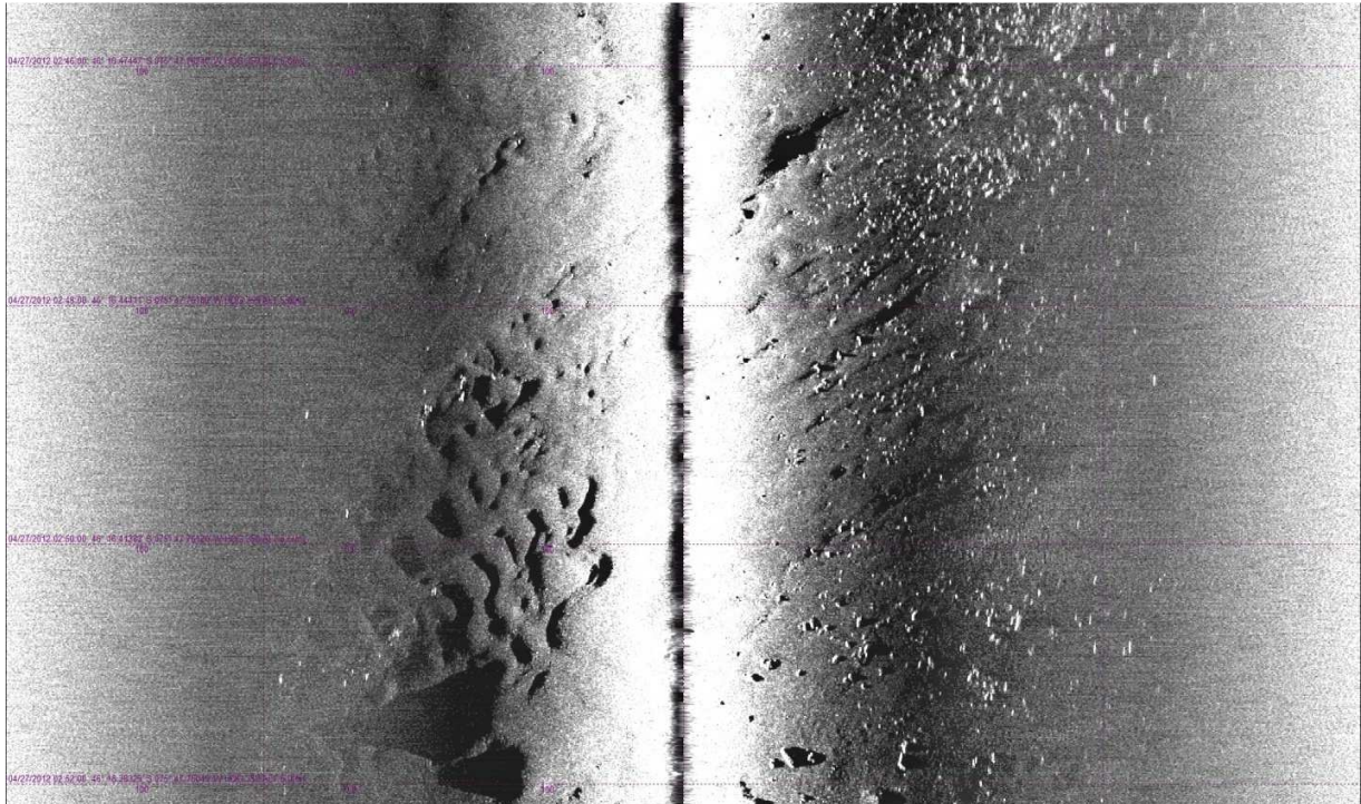
Figure 20 - Image from a steep side hill with the sidescan. This is a typical format for the standard data product (Image from Donna Blackman)
